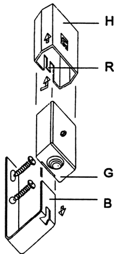
Fig. 2. Mounting
