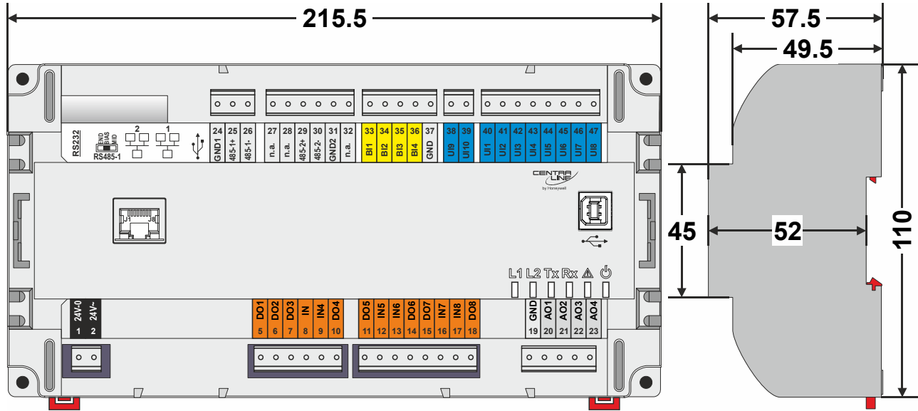
Fig. 9. EAGLEHAWK NX controller (w/o HMI but with RJ45 socket for connection of portable HMI, and with full complement of onboard I/Os), dimensions (in mm)
