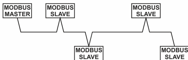
Fig. 6. Allowed Modbus wiring topology
