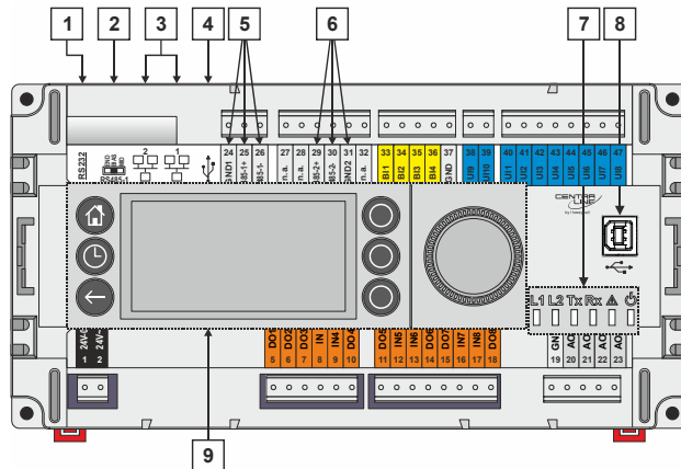
Fig. 3. Top view (with HMI and full complement of onboard I/Os)
