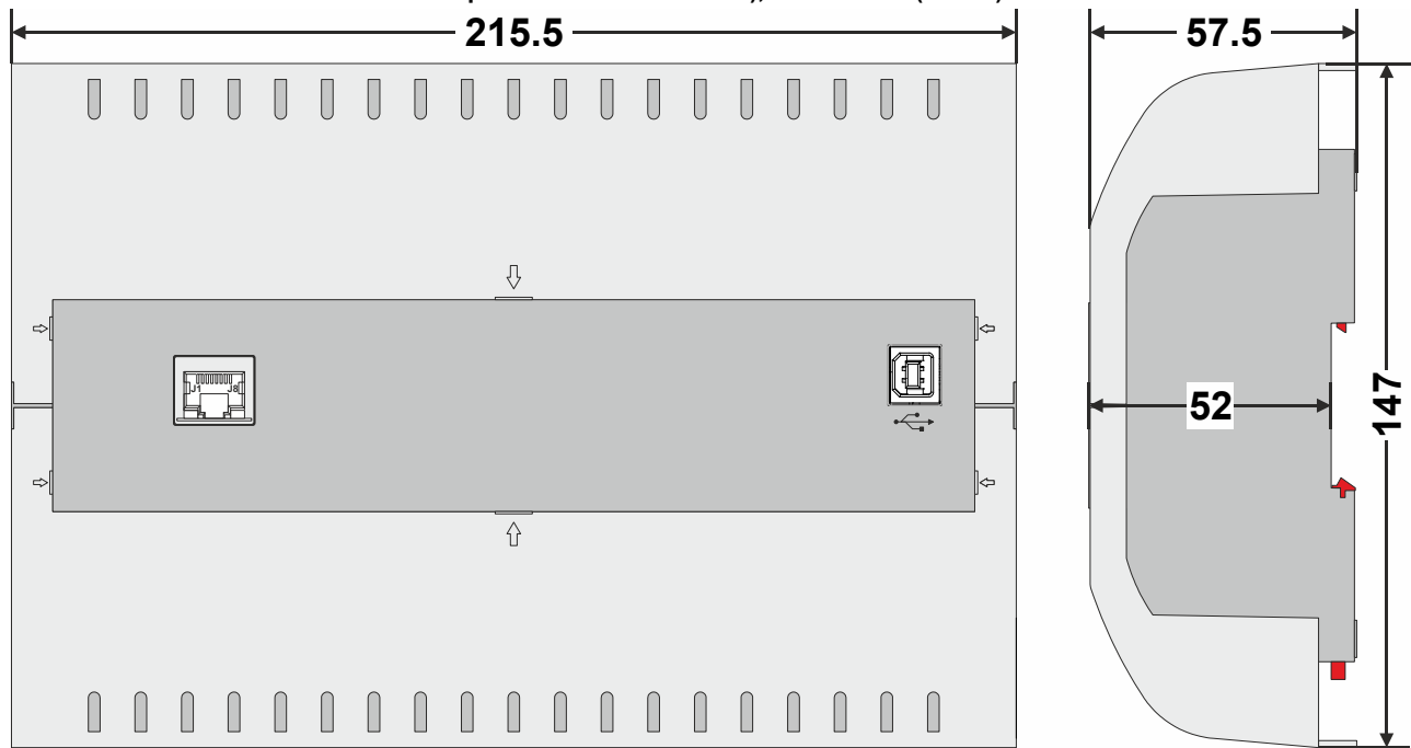
Fig. 10. EAGLEHAWK NX controller with covers, dimensions (in mm)
